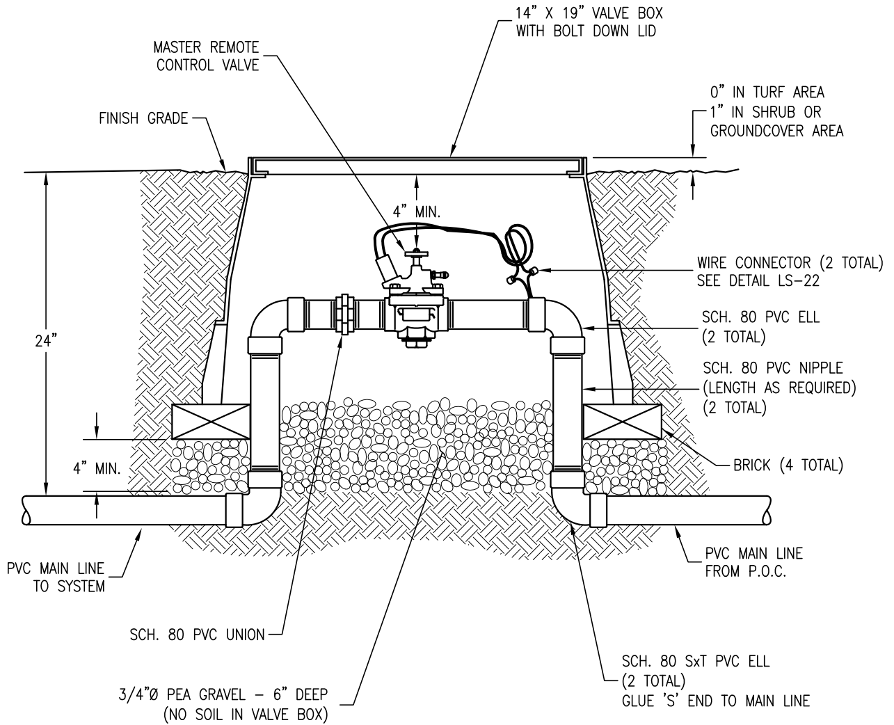
ELEVATION VIEW NO SCALE
